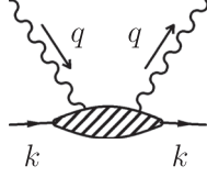
FIG. 1. Forward scattering of virtual photon of momentum q^\mu on a hadron of momentum k^\mu .
