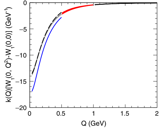
FIG. 11. Same as Fig. 8, but with W_1(0, Q^2) at low Q^2 taken as W_1(0, Q^2)^{\text{SIFF}} with dipole nucleon form factors and deviation from W_1(0, Q^2)^{\text{SIFF}} given by the band in Fig. 10.
