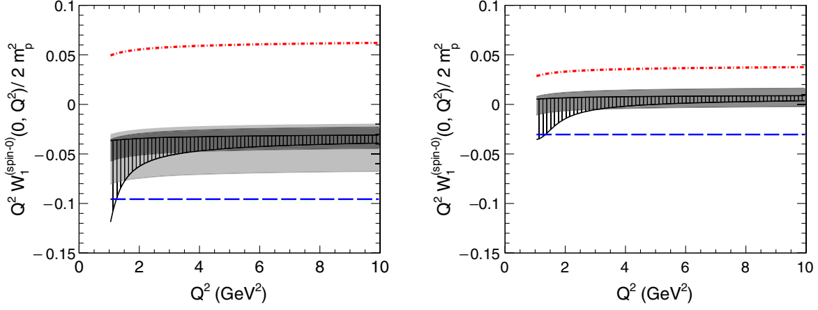
FIG. 4. Spin-0 contribution to Q^2 W_1(0, Q^2)/2m_p^2 as a function of Q^2 . The final results are given with n_f = 4 in the left-hand plot. For comparison, results with n_f = 3 are in the right-hand plot. The black band with vertical stripes displays the result with perturbative uncertainty estimated by renormalization scale variation Q/2 < \mu < 2Q . The solid bands represent hadronic uncertainty from local matrix elements in Table I. In the n_f = 4 evaluation, dark and light solid bands are obtained using f_c^{(0)} (pQCD) and f_c^{(0)} (lattice), respectively. The bottom dashed blue line and top dash-dotted red line give the separate quark and gluon contributions to the central value.
