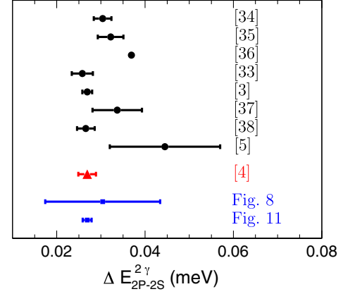
FIG. 9. Two-photon contribution to the Lamb shift in muonic hydrogen, adjusted to common proton elastic form factors (see the text). Black circles denote previous work, and the blue square denotes the present work. The red triangle is the summary of Ref. [4] used in the CREMA muonic hydrogen extraction of r_E^p .
