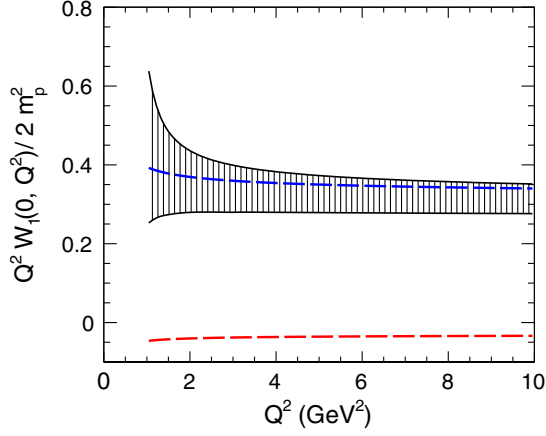
FIG. 6. Total Q^2 W_1(0, Q^2)/2m_p^2 as a function of Q^2 . The dashed red and blue lines denote central values for the spin-0 and spin-2 contributions. The vertical hatched black band is the total contribution, with perturbative and hadronic errors from each of the spin-0 and spin-2 contributions added in quadrature.
