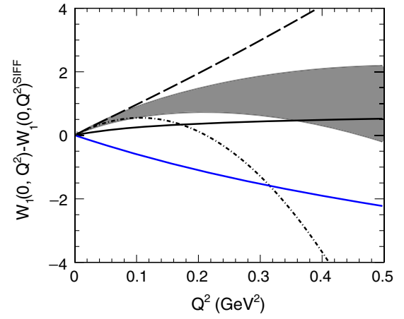
FIG. 10. Different calculations of W_1(0, Q^2) - W_1(0, Q^2)^{\text{SIFF}} . The black solid line, black dashed line, and solid band, give the “third-order” ( \bar{T}_1^{(3)} ), “fourth-order” ( \bar{T}_1^{(3)} + \bar{T}_1^{(4)} ), and “fourth-order plus \Delta ” ( \bar{T}_1^{(3)} + \bar{T}_1^{(4)} + \bar{T}_1^{(\Delta)} ) results of Ref. [3], using the parameters of Ref. [3] and their prescription for determining \delta\beta . The solid band adds in quadrature the errors from c_1, c_2, c_3, \beta , and g_{\pi N\Delta} . The dash-dotted black line gives the fourth-order plus \Delta contribution ( \bar{T}_1^{(3)} + \bar{T}_1^{(4)} + \bar{T}_1^{(\Delta)} ), Taylor expanded through \mathcal{O}(Q^4) . The bottom blue solid line gives the “third-order” [ T_1^{(\text{NB})}(0, Q^2) ] result of Ref. [38], using its parameters.
