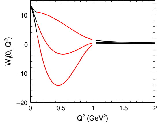
FIG. 7. W_1(0, Q^2) as a function of Q^2 . Solid black curves on the left and right are from Eqs. (33) and (35), as explained in the text. Intermediate red curves are interpolations from the central curves and envelopes.
