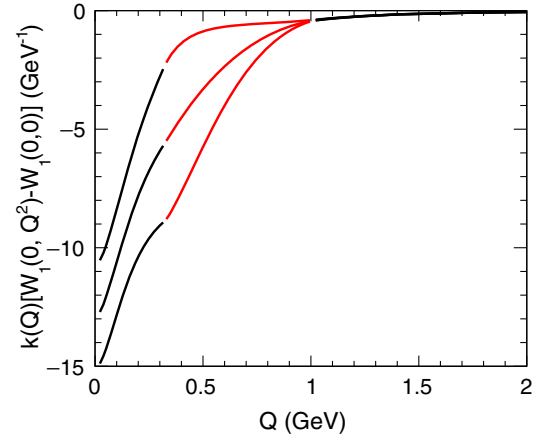
FIG. 8. W_1(0, Q^2) , after subtracting the Q^2 = 0 limit and scaling by the kinematic factor k(Q) in Eq. (38), as a function of Q . The contribution to the muonic hydrogen Lamb shift is proportional to the area under the curve, cf. Eq. (37).
