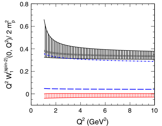
FIG. 5. Spin-2 contribution to Q^2 W_1(0, Q^2)/2m_p^2 as a function of Q^2 . The dark gray band represents hadronic uncertainty. The vertically hatched band represents perturbative uncertainty, estimated by varying renormalization scale Q/2 < \mu < 2Q . Upper dash-dotted and lower dashed blue lines represent the contributions of the up quark and down quark to the central value, and the lower red hatched band shows the gluon contribution and uncertainty.
