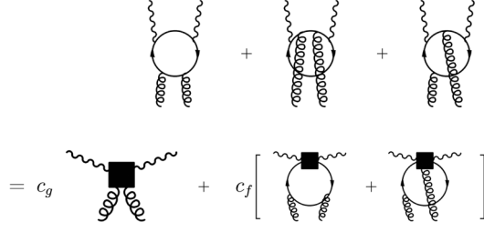
FIG. 3. Matching condition onto gluon operators. The three diagrams on the left-hand side denote the contributions T_a^{\mu\nu} , T_b^{\mu\nu} , and T_c^{\mu\nu} in Eq. (10). The right-hand side denotes a sum over operators in Eq. (7). Permutations of external states are not displayed.
